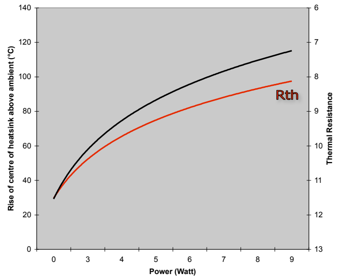
HeatSink Performance
