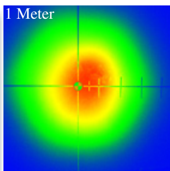
KEPL2425 (25°) Spectro Metric Analysis
