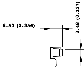
Detail A Scale 3:1
