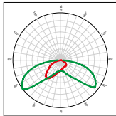
PLAL0155 IESNA Type III Full angle at 50% from maximum: ~ 160° x 130° Full angle at 10% from maximum: ~ 175° x 155°
