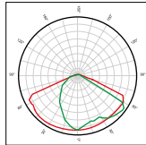
VIA2X3/5050T3 IESNA Type III Medium
