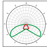
PLAL0133 IESNA Type I Full angle at 50% from maximum: ~ 150° x 90° Full angle at 10% from maximum: ~ 160° x 100°
