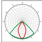
PLL2091EW Full angle at 50% from maximum: ~ 60° Full angle at 10% from maximum: ~ 100°
