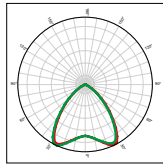
PLAL0122 90° FWHM Full angle at 50% from maximum: ~ 90° Full angle at 10% from maximum: ~ 95°
