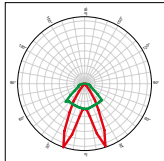
PLL2091AX Full angle at 50% from maximum: ~ -30/+30° Full angle at 10% from maximum: ~ 90°
