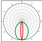
RYO/NA Full angle at 50% from maximum: ~ 20° Full angle at 10% from maximum: ~ 80°
