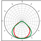
RYO/UW Full angle at 50% from maximum: ~ 90° Full angle at 10% from maximum: ~ 150°
