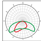
PLAL0177 ME3A Full angle at 50% from maximum: ~ 155° x 120° Full angle at 10% from maximum: ~ 165° x 140°
