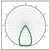
PLAL0111 60° FWHM Full angle at 50% from maximum: ~ 60° Full angle at 10% from maximum: ~ 75°
