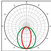
RYO/EW Full angle at 50% from maximum: ~ 55° Full angle at 10% from maximum: ~ 120°
