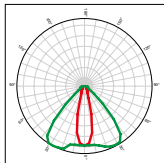
PLL2091WI Full angle at 50% from maximum: ~ 30° Full angle at 10% from maximum: ~ 90°
