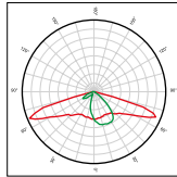
VIA2X3/5050T2MC IESNA Type II Medium
