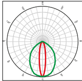
RYO/ME Full angle at 50% from maximum: ~ 30° Full angle at 10% from maximum: ~ 95°
