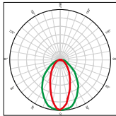
RYO/WI Full angle at 50% from maximum: ~ 45° Full angle at 10% from maximum: ~ 110°
